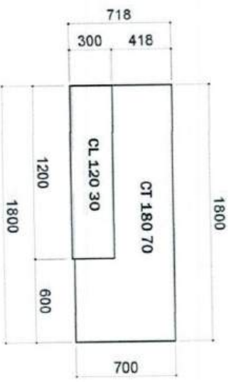
PLAN
