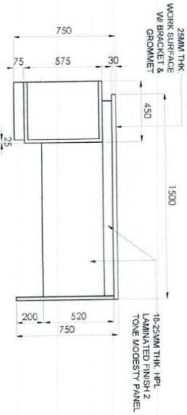
FRONT ELEVATION
