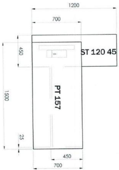
PLAN
