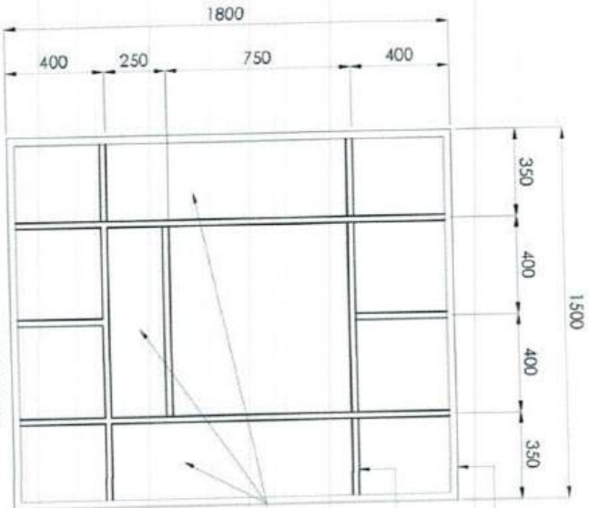
FRONT ELEVATION
