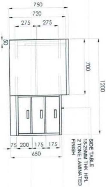
SIDE ELEVATION
