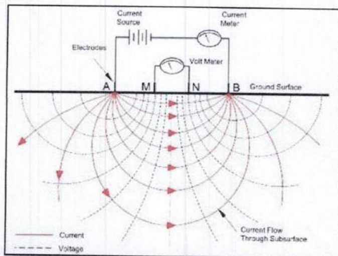
Figure 1: Generalized Movement and Direction of Voltage and Current During a Resistivity Reading
