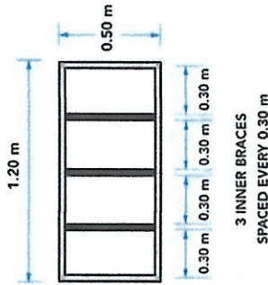
SHELF BRACING DETAIL (TOP VIEW OF EACH SHELF)
